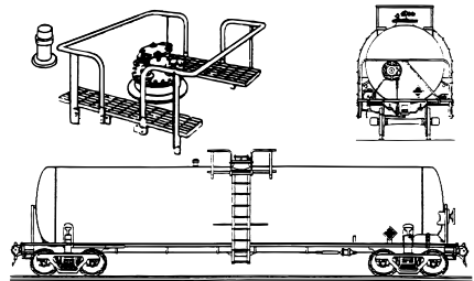
Low Pressure Tank Car Liquids (Closed Dome and Outlets on top) (131)
